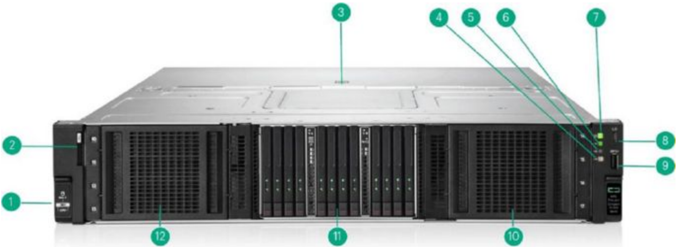
Front View - GPU chassis
